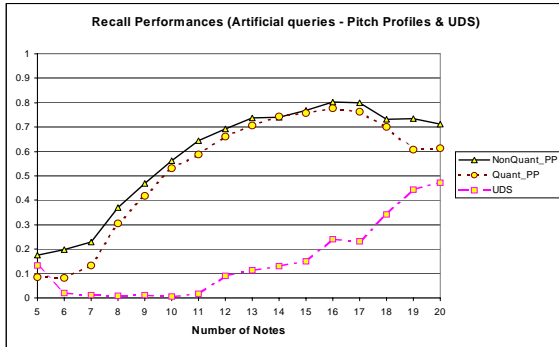
Figure 4: Recall performances of three melodic comparison engines stimulated by artificial queries.
